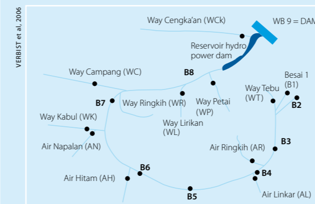
Figure 2. Sketch of the main rivers in the Sumber Jaya Basin and the locations where sediment loads were measured.
